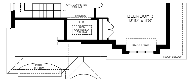
PARTIAL SECOND FLOOR PLAN ELEV. C
