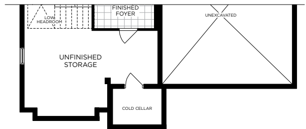
PARTIAL BASEMENT PLAN ELEV. C
