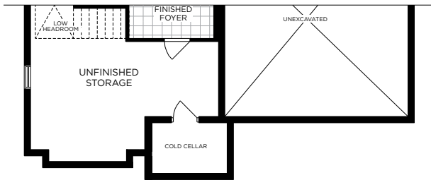
PARTIAL BASEMENT PLAN ELEV. B
