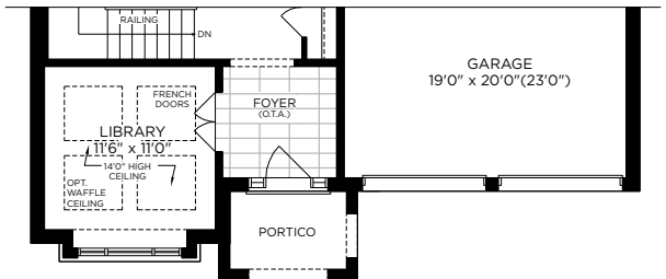
PARTIAL GROUND FLOOR PLAN ELEV. B
