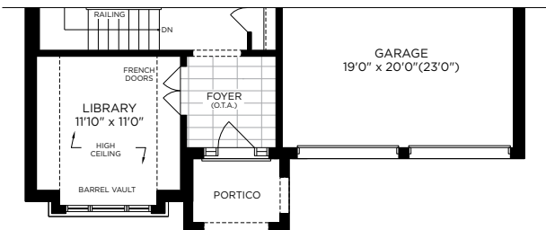
PARTIAL GROUND FLOOR PLAN ELEV. C
