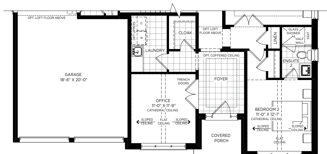
GROUND FLOOR ELEVATION B
