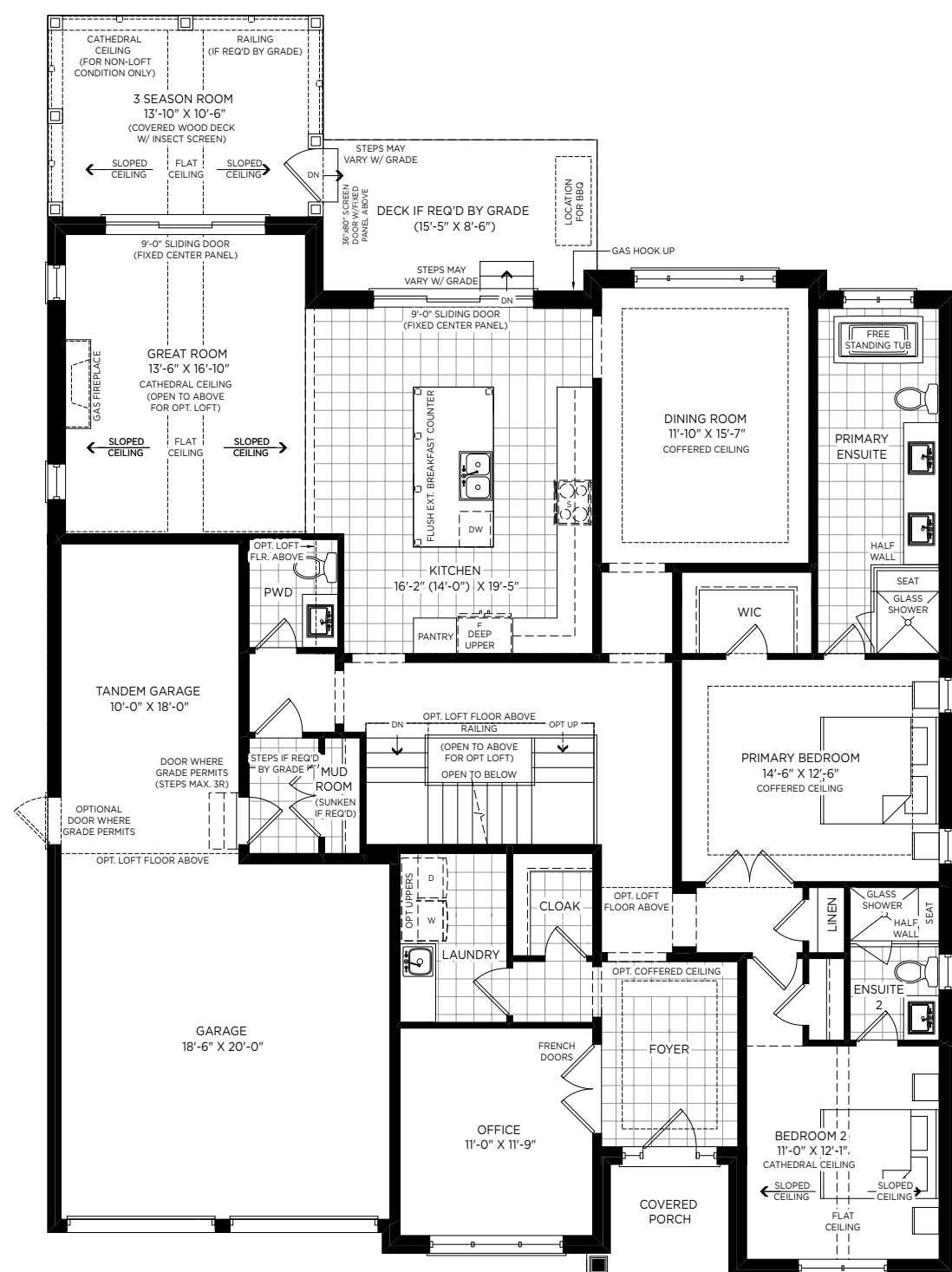
GROUND FLOOR ELEVATION A
