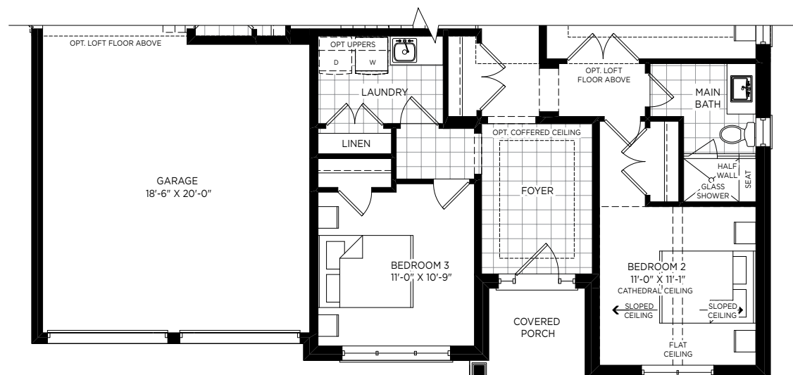
OPT. GROUND FLOOR WITH THIRD BEDROOM ELEVATION A
