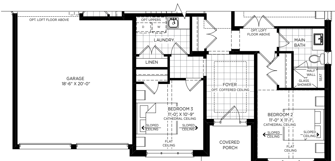
OPT. GROUND FLOOR WITH THIRD BEDROOM ELEVATION B
