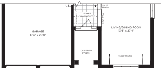
GROUND FLOOR, ELEVATION B
